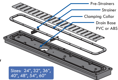
Cross-Hatch Strainer
